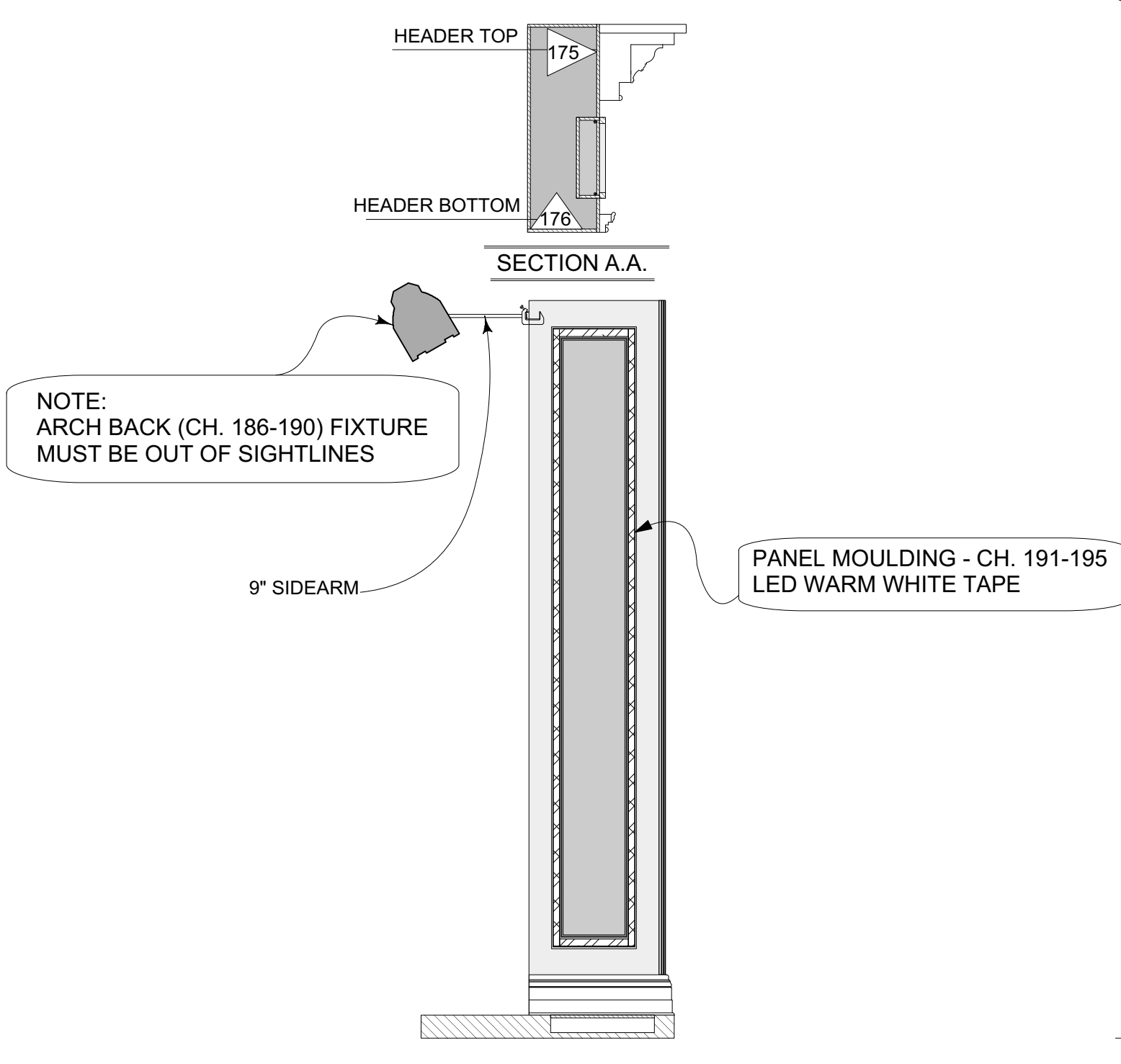
TYPICAL SECTION
